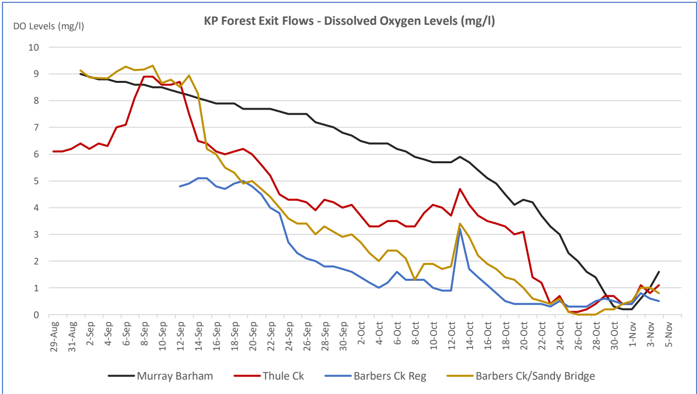
Figure 2: K-P Forest exit flow depths (m) & dissolved oxygen levels (mg/l)
